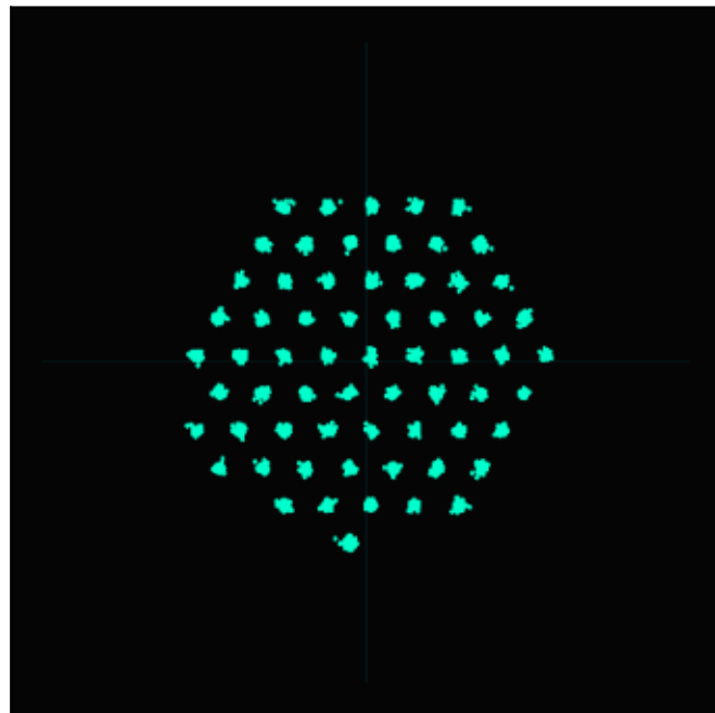
64-HQAM (hexagonal)
