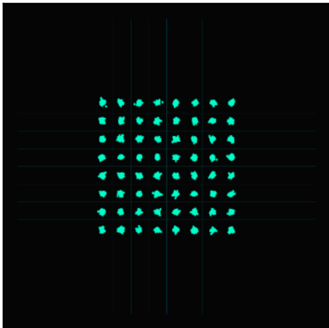
64-QAM (square)
